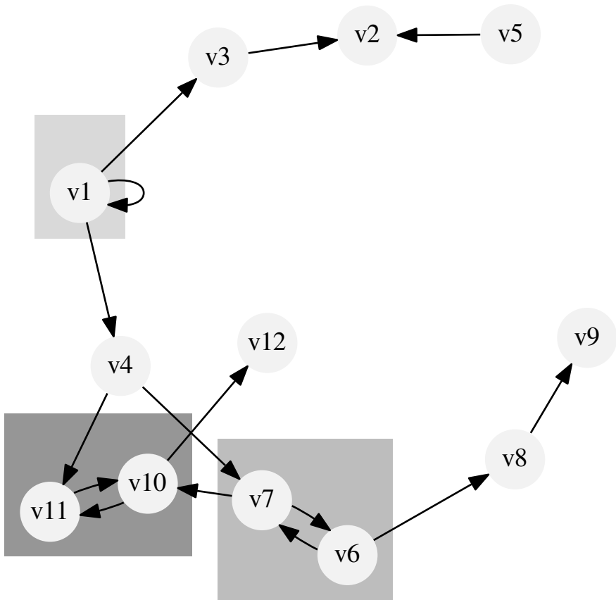
Example 6: Interaction graph with SCC style
