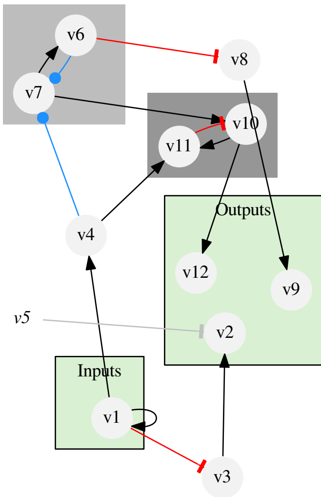
Example 10: Interaction graph with default style
